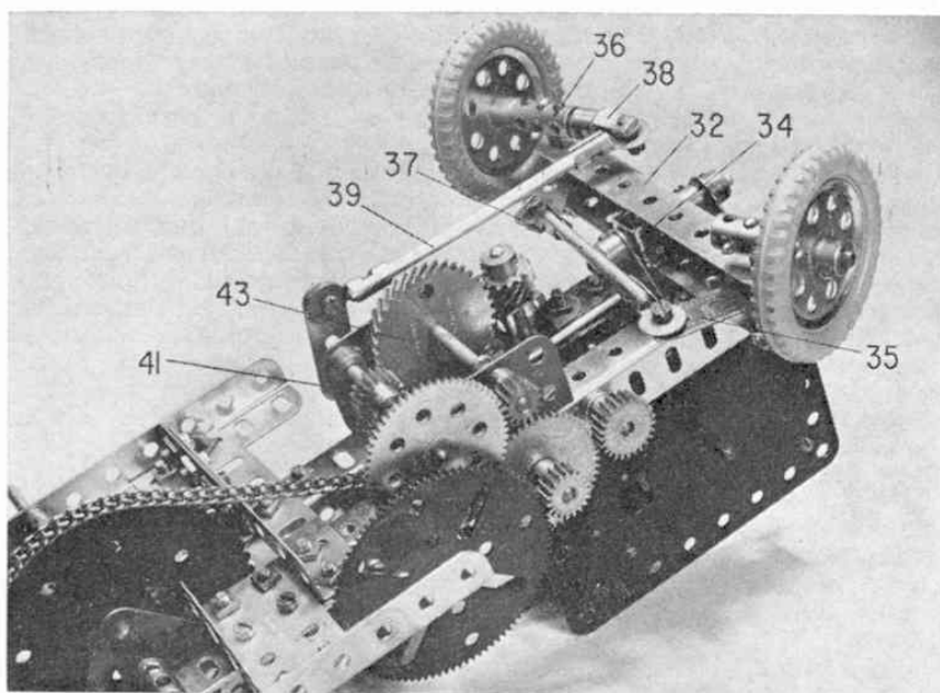
Top, full credit for this smooth-running Agricultural Tractor goes to Mr David Cowdrey of Weston Turville, Aylesbury, Bucks. Left, in this close-up underside view of the forward section of the model the layout of the drive and steering systems is clearly shown.
