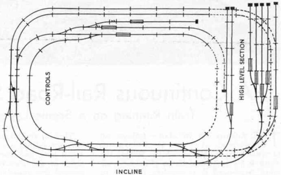
Peter Barr's layout requires the following rails, etc.: 22 EDA1; 2 EDAT1, 7 EDA2; 1 EDAT2; 13 EDA1½; 65 EDB1; 22 EDB1½; 6 EDB1¼; 2 IBR½; 2 Switches D2; 9 UBR; 2 Diamond Crossings Right-hand, EDCR; 4 EODPR; 7 EODPL; 10 Switches D1; 2 ISPR; 4 ISPL; 9 Buffer Stops D1.
