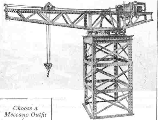
Hammer-Head Crane
