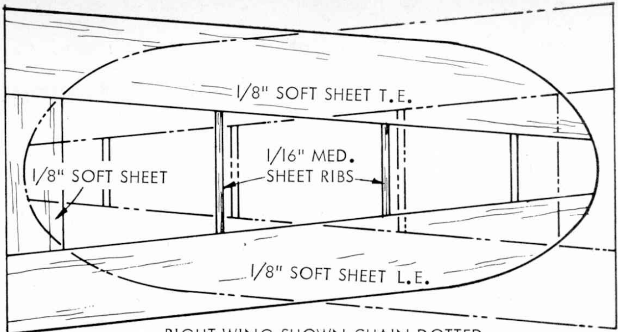
WING RIB SECTION
