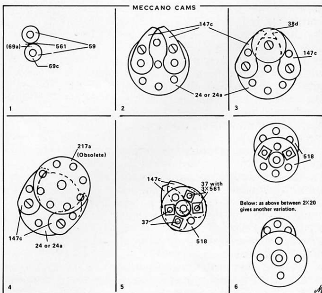
TOP CENTRE: Pierre Couroble's Roller Bearing design.
