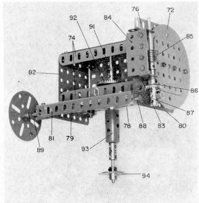
The universal milling head removed from the model. Note that, when in place, Contrate 92 meshes with Pinion 95 on Rod 32.
