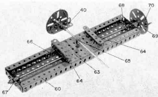
In this underside view of the worktable and saddle, the method of obtaining traverse- and cross-feed is clearly shown.
