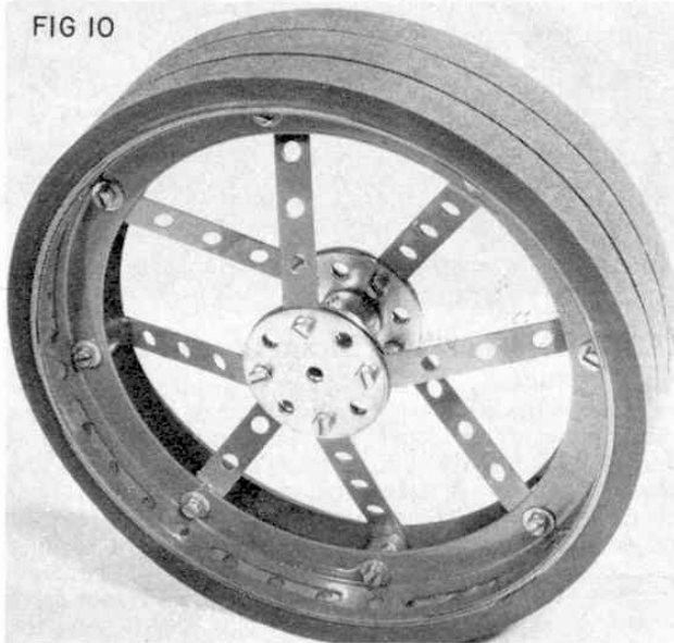
Fig. 10: A partially-completed dished spoked wheel for a traction engine using 2½ in. Narrow Strips for spokes. Eight-hole Wheel Discs are used to "sandwich" the spokes.
