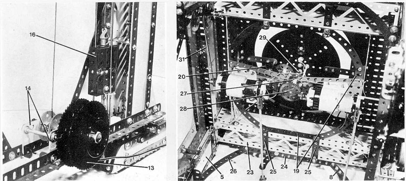
Fig. 6, above left, shows the cable drum mounting of the No. 10 Set Electric Dockyard Crane. Reinforced Plastic Plates give insulated feed for the flexible cable and note the counterweight giving automatic reel-in. Fig. 7, above right, is a view from beneath the tower platform showing the mounting for travelling and slewing motors. Note transverse reinforcing provided by 12½" Braced Girders.
