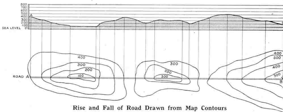
Rise and Fall of Road Drawn from Map Contours
