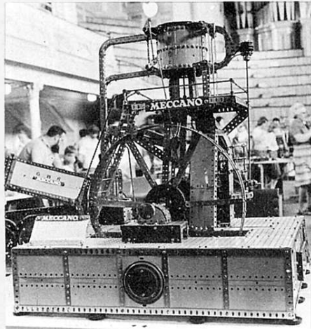
Above left, another superb Traction Engine was "Rosie" by Geoff Coles, the smallest model of its type we have seen with full working features. Above centre, a Vertical Mill Engine by Harry Wolfenden. Above right, an unusual Vertical Table Meccanograph built by Dave Barton from an original design by Andreas Konkoly of Hungary. Below left, Mike Pashley's enormous W1800 Walking Dragline - always a big attraction. Below right, Mike Cotterill pictured with his Schools Class 4-4-0 Locomotive, recalling the romantic days of live steam.
